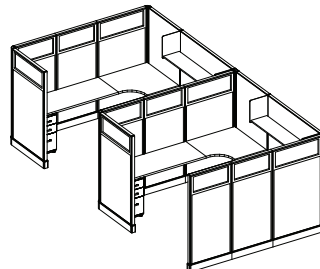
OFD-U2-67GPN-8X8C-2 67"H 2-Pod Workstation 8'x8' NON-POWERED Workstations, includes Partial-Glazed Panels, BBF, Lateral File, and 60" Full-shelf per Station List $28,865 List per Station $14,433
