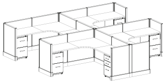
OFD-U2-39N-6X6C-4 39"H 4-Pod Workstation 6'x6' NON-POWERED Workstations, includes a BBF and FF Pedestal per Station List $27,030 List per Station $6,758
